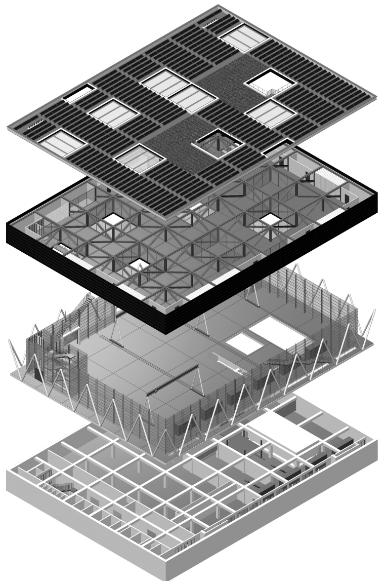
explosionsisometrie
